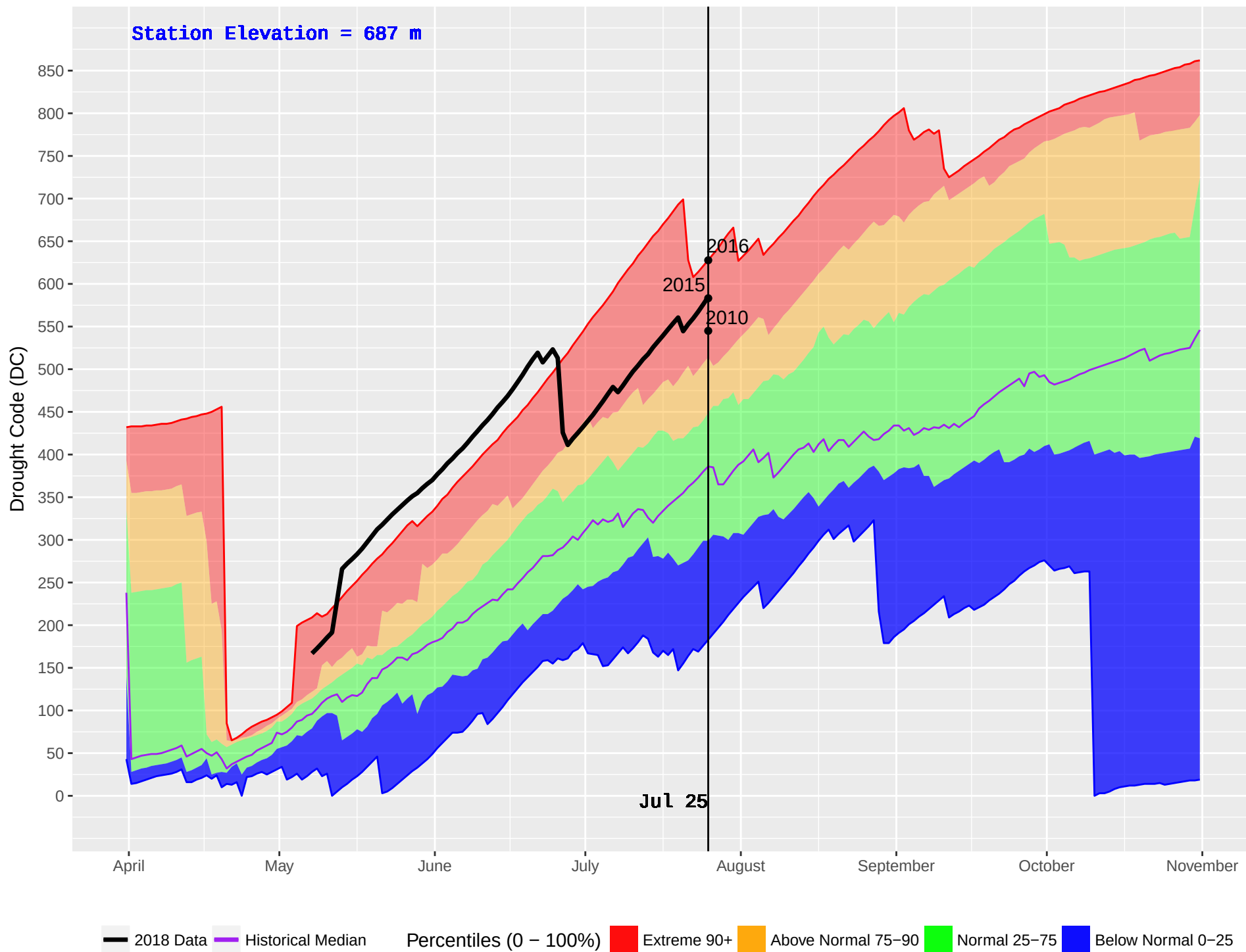
KETCHIKA (444) : Historical (1986–2016) and Current (2018) Noon Drought Code (DC)
