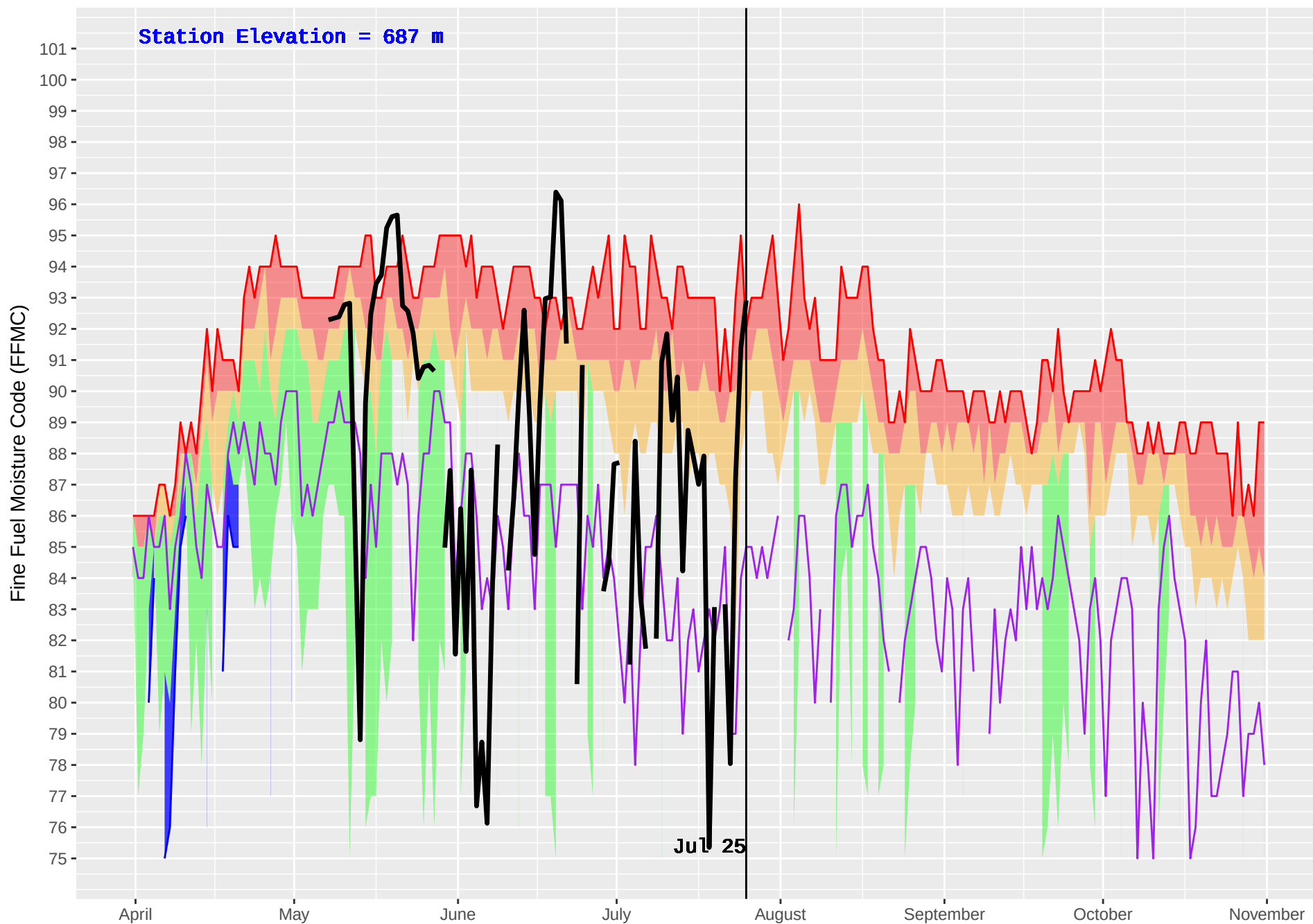
KETCHIKA (444) : Historical (1986–2016) and Current (2018) Noon Fine Fuel Moisture Code (FFMC)
