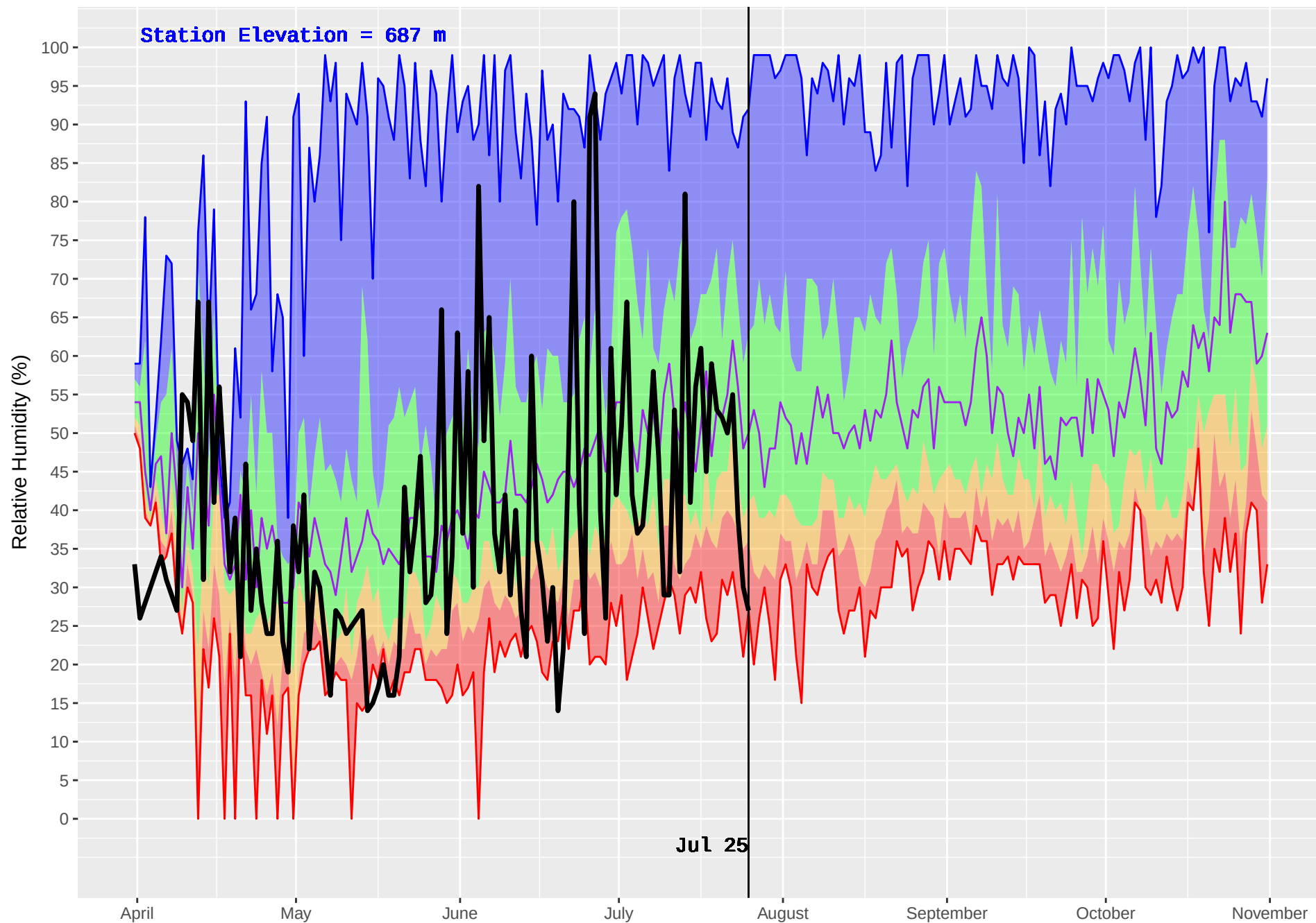
KETCHIKA (444) : Historical (1986–2016) and Current (2018) Noon Relative Humidity
